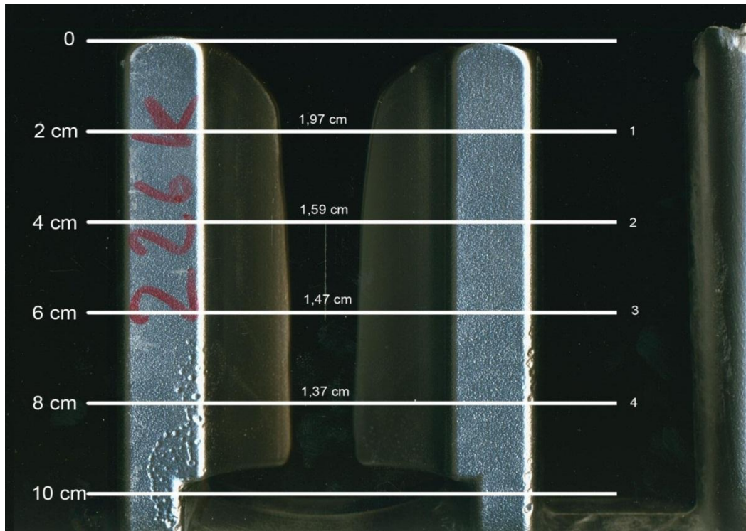
Figure 3.10 Measurement of gaps in Bolt Test
